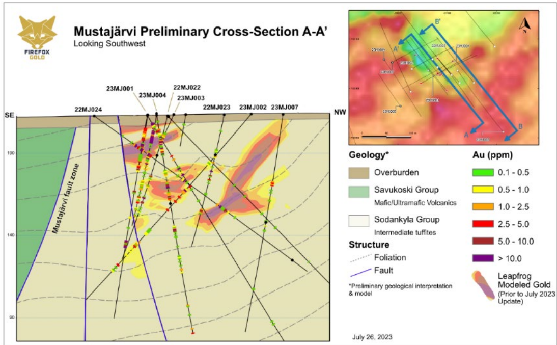
Figure 11. Preliminary Cross Section through East Target Looking SW (23MJ001 and 002)
