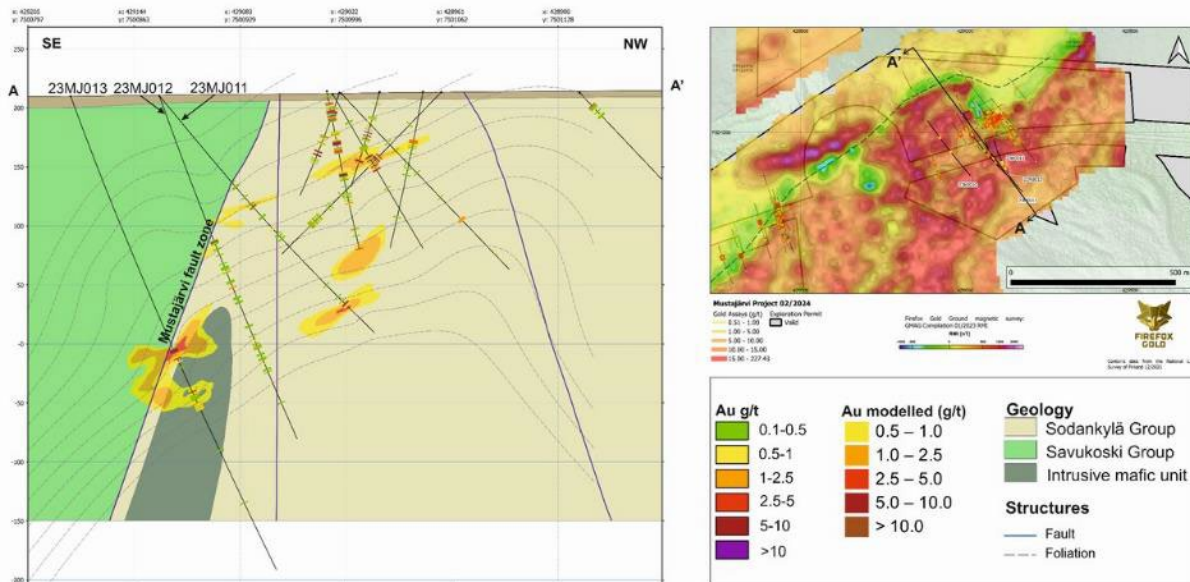
Figure 14. West facing cross-section showing the drill hole fence 23MJ013-23MJ011 and the interpreted mineralization along the section plan A-A'.
