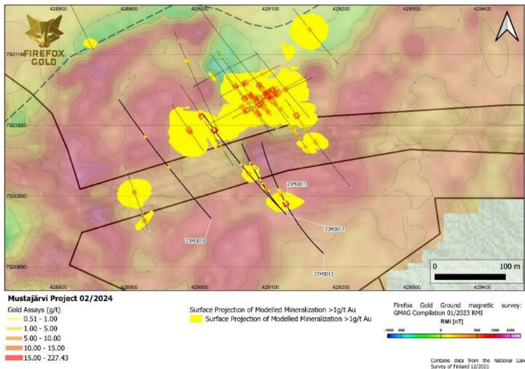
Figure 13. Plan view of Mustajärvi East drilling with autumn 2023 drilling highlighted. Modeled gold shapes projected to surface are up-to-date for the MD&A Q4 of 2023.
