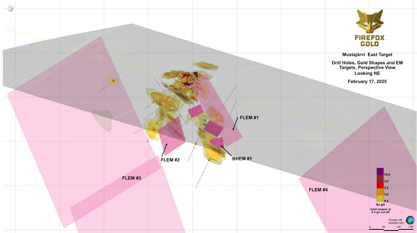
Figure 19. 3D perspective view of Mustajärvi East gold shapes (looking NE) with EM targets.
