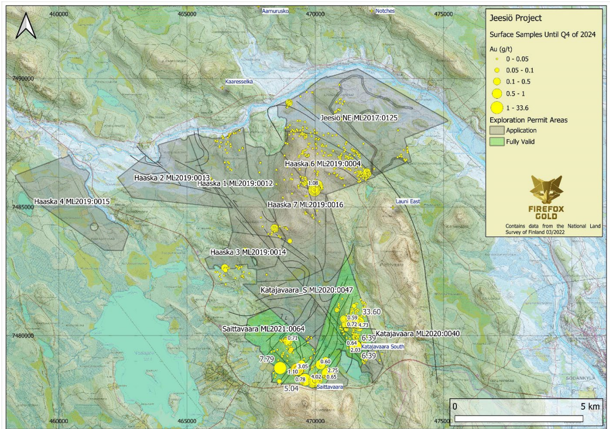
Figure 1 - Jeesiö property with all the gold-assayed surface rock samples until the end of 2024.
