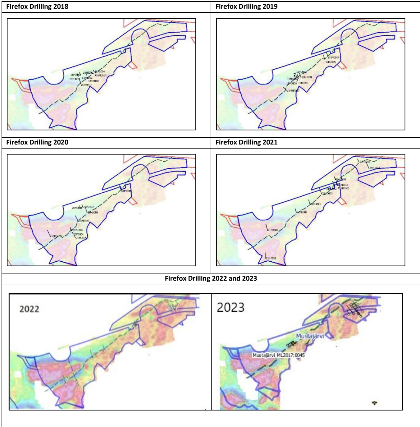
Figure 5. Phases of drilling at Mustajärvi; drill holes from 2018 to 2023
