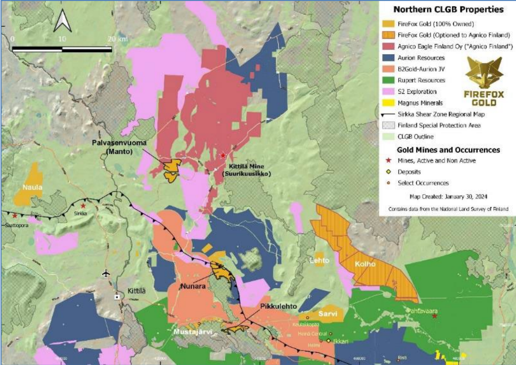
Figure 25. Map figure highlighting Palvasenvuoma, Nunara and Pikkulehto (Mustajärvi Project) properties.
