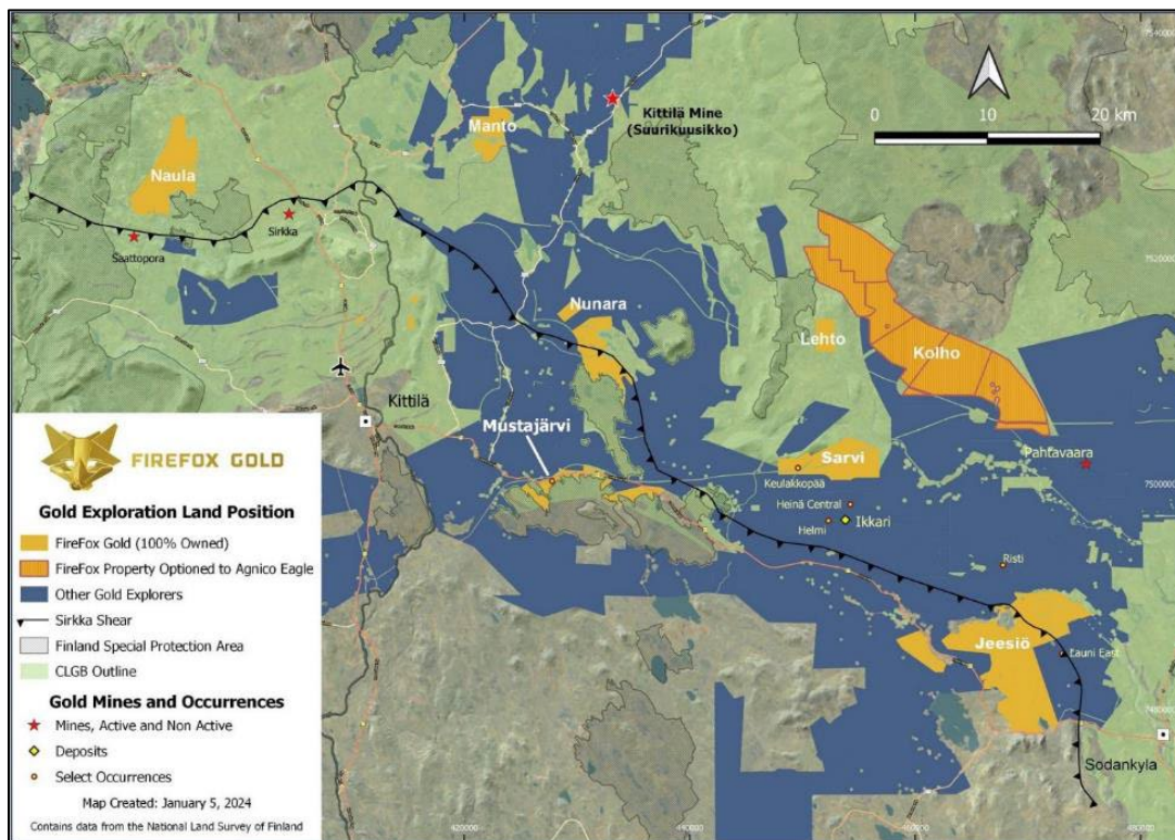
Figure 20. Current FireFox properties in Lapland, starting from left: Naula, Manto, Mustajärvi, Nunara, Sarvi, Kolho (optioned to Agnico Eagle) and Jeesiö.
